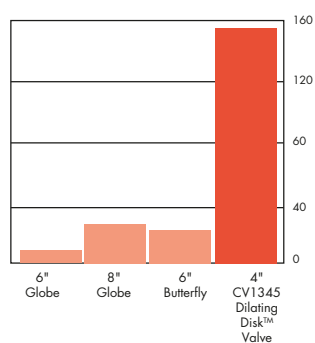
Rangeability
