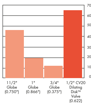
Volumetric Flow Rate ( \Delta P=10 psid) (US GPM)
