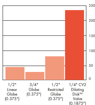
Rangeability
