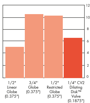
Volumetric Flow Rate ( \Delta P=10 psid) (US GPM)
