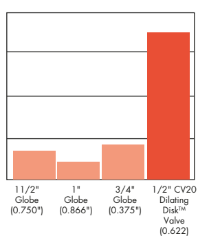
Rangeability
